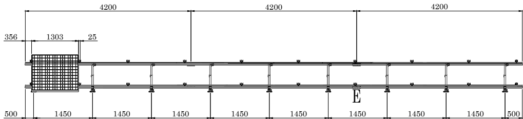
VISTA FRONTAL
