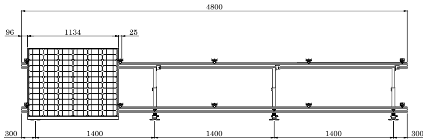
VISTA FRONTAL
