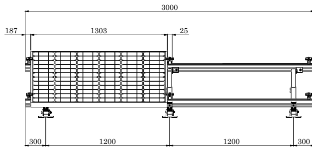
VISTA FRONTAL
